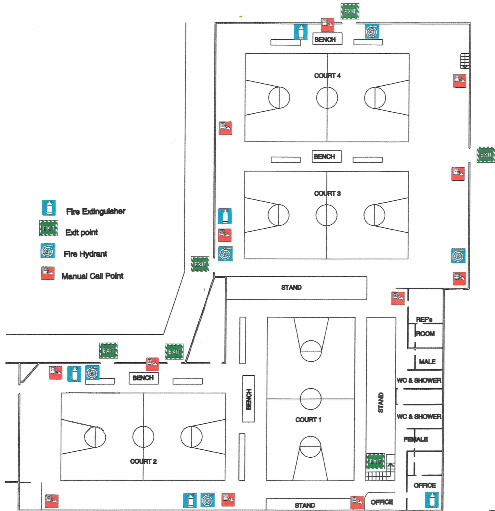
GROUND FLOOR
